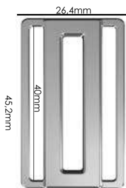
Ref.: AMP 093 40mm
