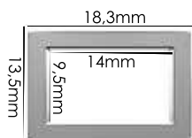
Ref.: AMP 069 14mmx 9,5mm Material: zamac
