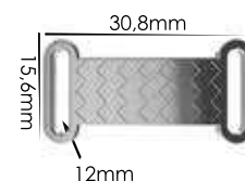
Ref.: AMP 049 12mm
