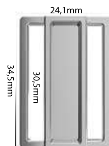
Ref.: AMP 100 30,5mm
