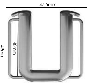
Ref.: AMP 062 40mm (Sob Consulta)
